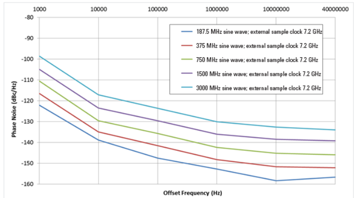
Phase noise plot with external sample clock, 7.2 GSa/s, direct output measured with balun
