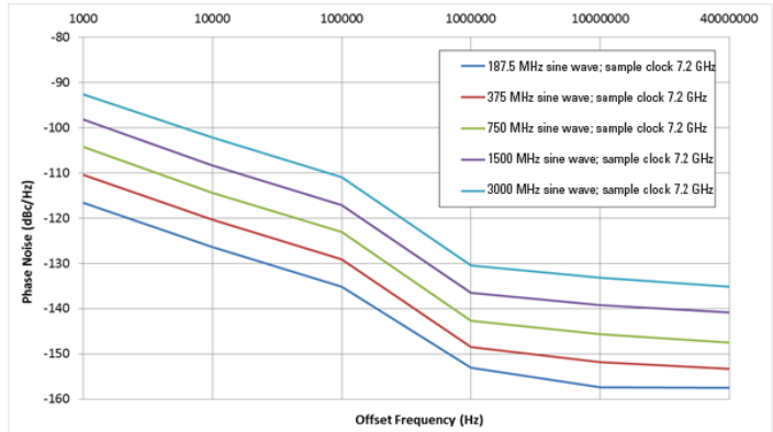
Phase noise plot with internal sample clock, 7.2 GSa/s, direct output measured with balun
