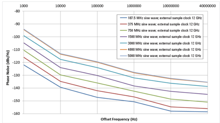
Phase noise plot with external sample clock, 12 GSa/s, direct output measured with balun
